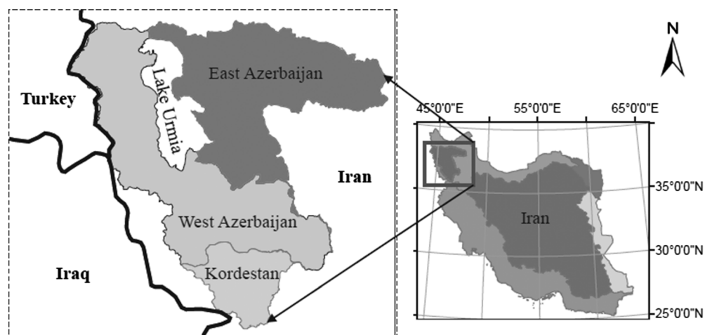
FIGURE 1 The location of Urmia Lake in Iran
